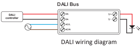
DALI wiring diagram
