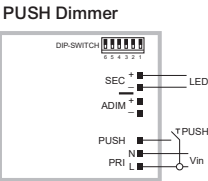
PUSH wiring diagram
