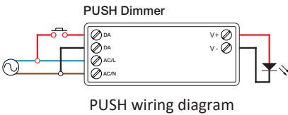
PUSH wiring diagram
